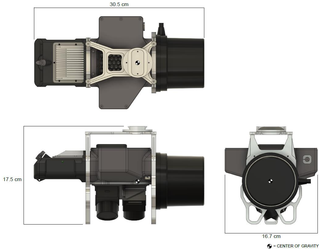
Figure 2: True View 515 dimensions with CG
